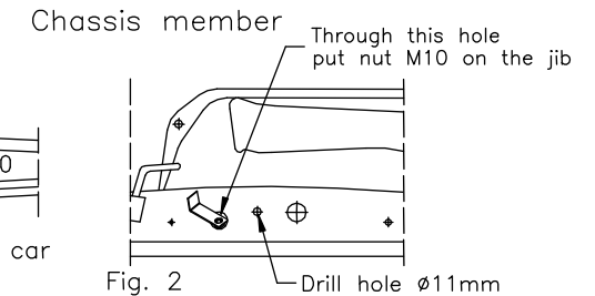
Fig. 2 Drill hole \phi 11 mm
